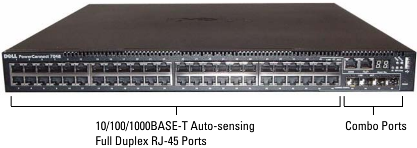
Figure 1-4. PowerConnect 7048 with 48 10/100/1000BASE-T Ports
