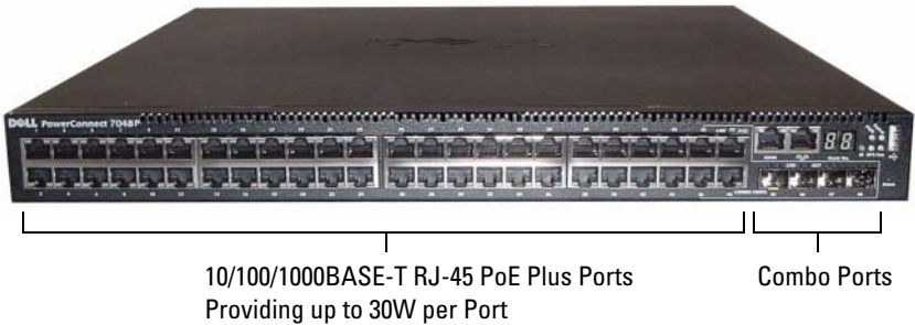
Figure 1-5. PowerConnect 7048P with 48 10/100/1000BASE-T PoE Plus Ports
